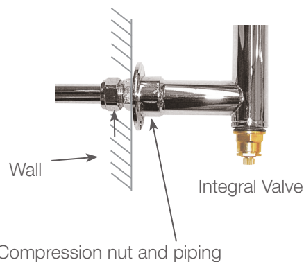
INTEGRAL COLLECTION VALVE FITTING
