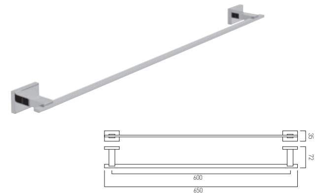
towel rail wall mounted 650mm (26")
