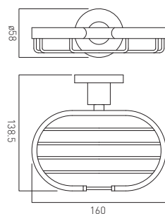
soap holder wall mounted
