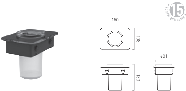
frosted glass tumbler with 150mm glass insert (for use with MUS-184-45 / MUS-184-60)
