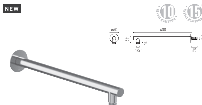
Safari easy fit shower arm wall mounted
