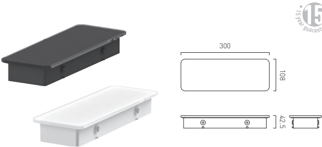
300mm glass shelf insert (for use with MUS-184-45 / MUS-184-60)
