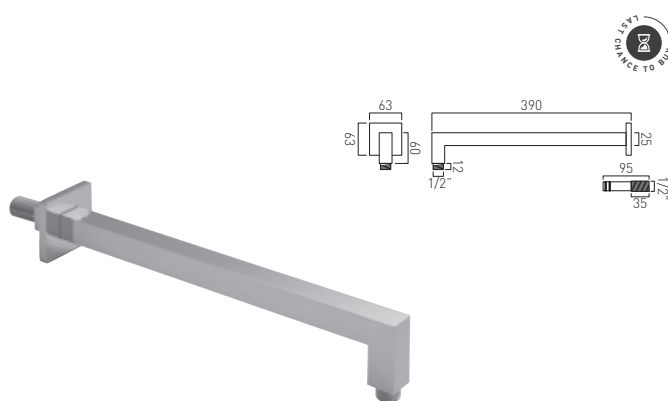
Mix² easy fit shower arm wall mounted
